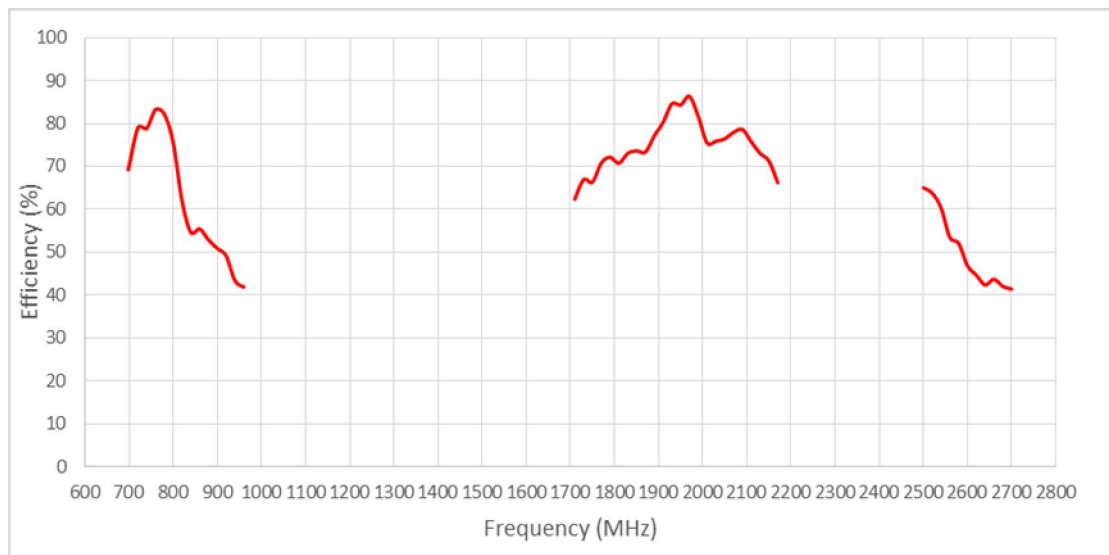
Efficiency (%)
